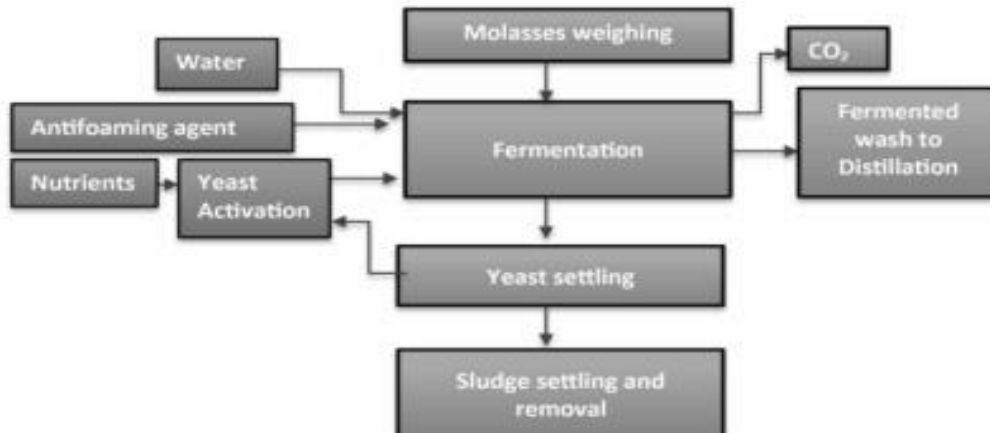
Figure 4 Fermentation Flow Chart
