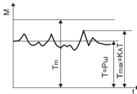
Fig. 1: Diagram of the Coupling Moment
