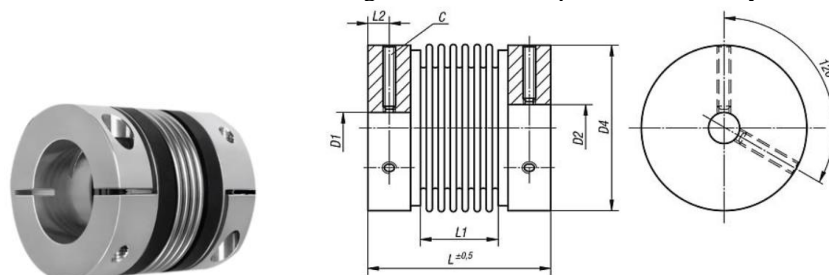
Fig. 21: Bellow Coupling
