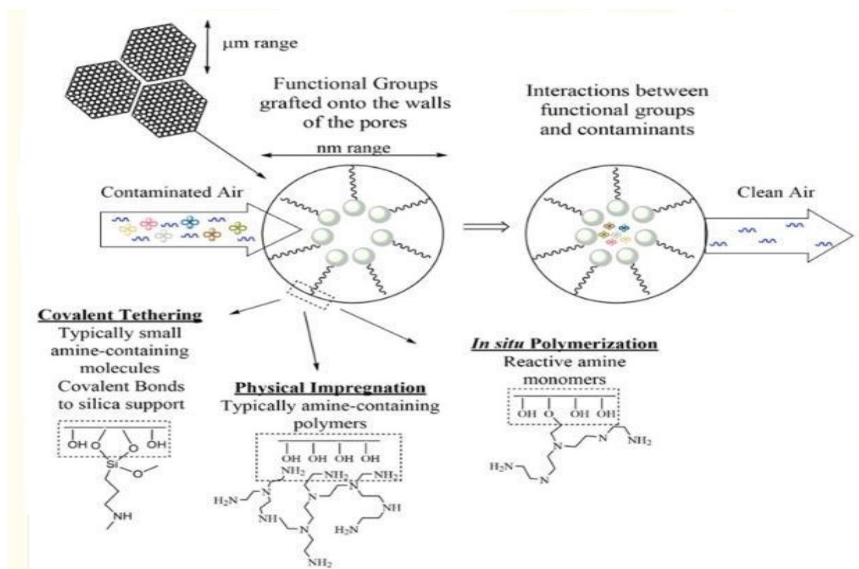
Figure-2: An example of mesoporous silica materials used for environmental remediation of contaminants.
