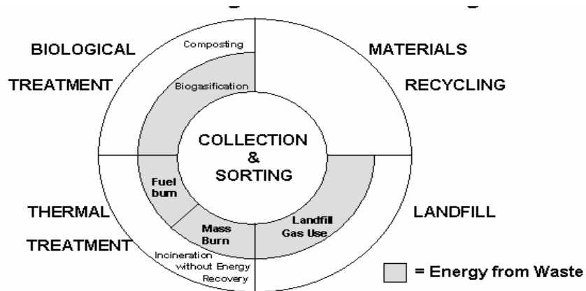
Fig. 1: Elements of Integrated Solid Waste Management [10] Image details size 10 bold italic center aligned
